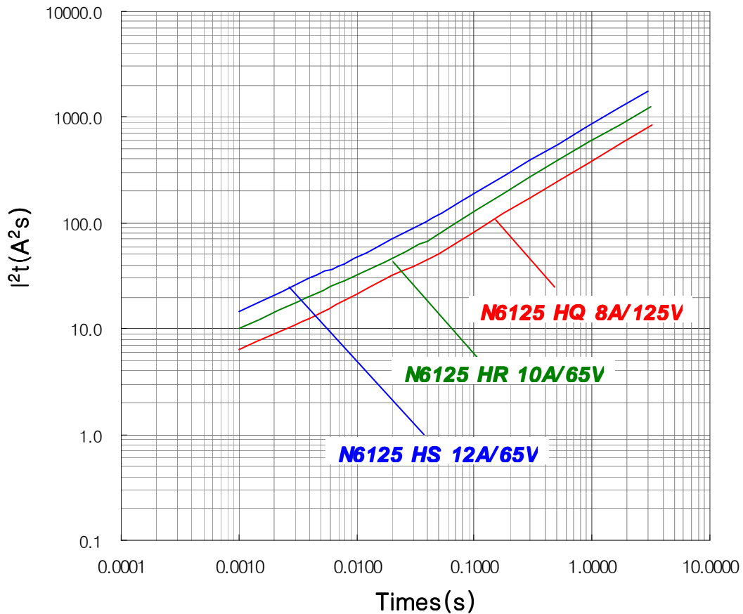
I 2 t vs.t Curves
